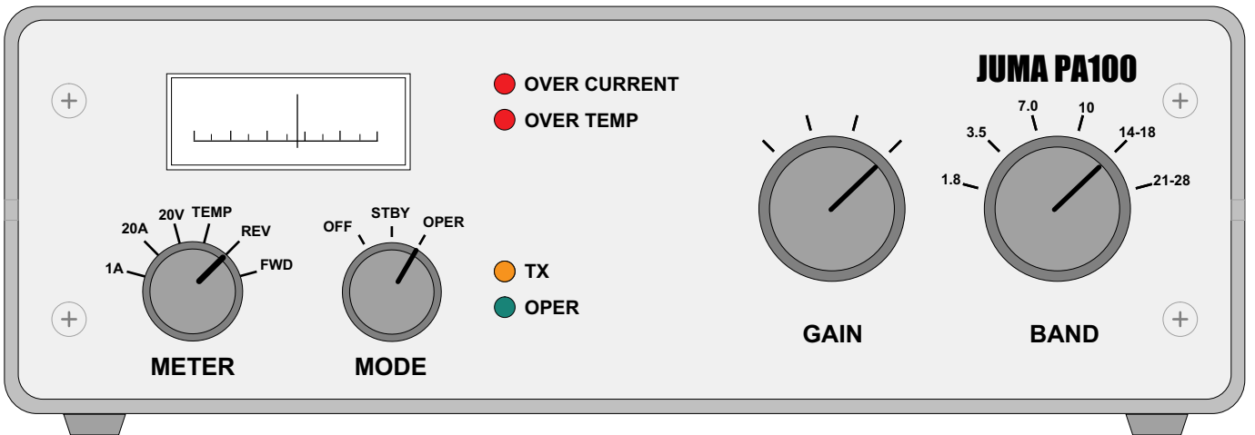
JUMA-PA100 LINEAR AMPLIFIER OH2NLT & OH7SV
