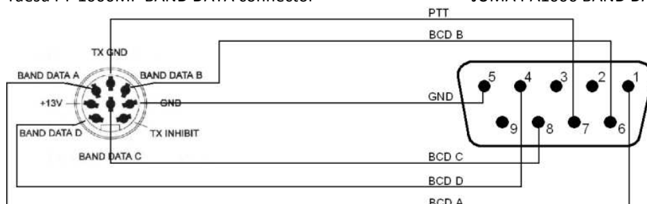
8 pin DIN male plug in cable
