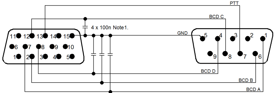
DB15 male plug seen from solder side
