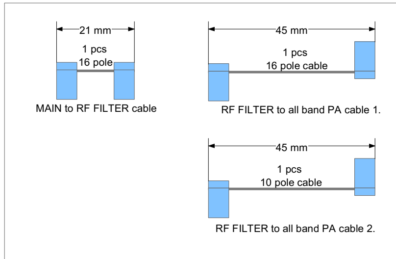
All band cables
