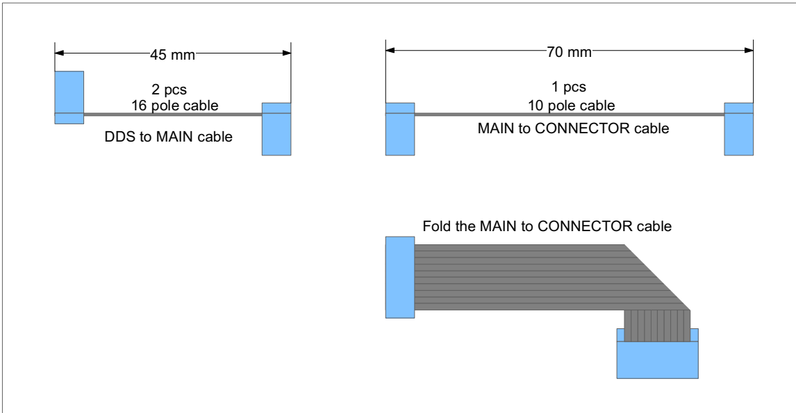
The base flat cables for all JUMA TRX2 models
