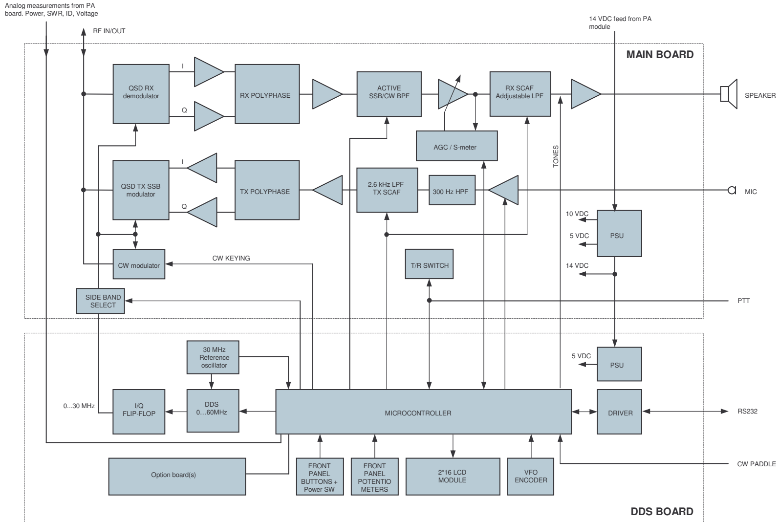
JUMA-TRX2 EXCITER BLOCK DIAGRAM
