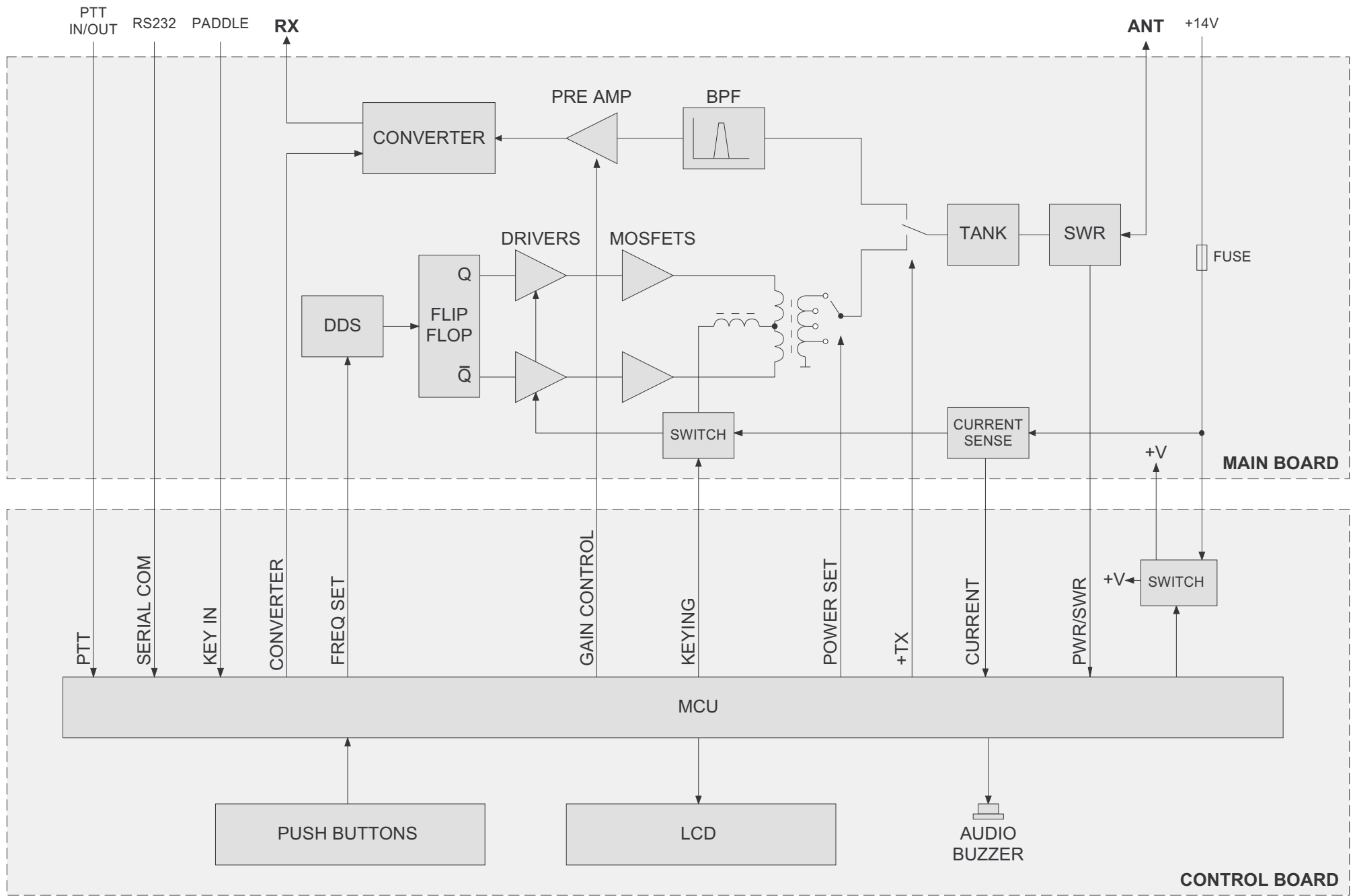
JUMA TX500 & TX136 block diagram 2009-09-10 OH2NLT & OH7SV
