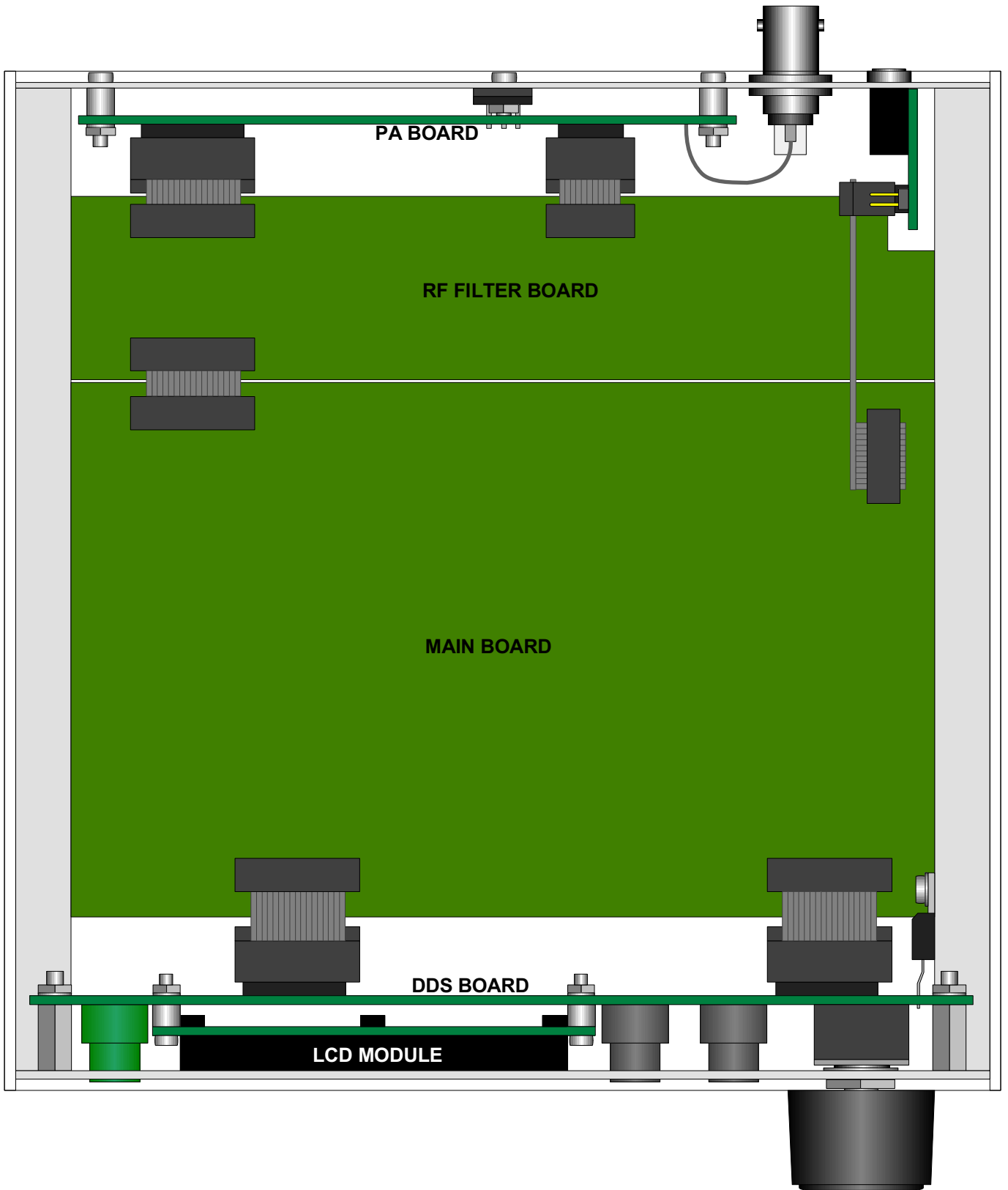
JUMA-TRX2 HF TRANSCEIVER All band construction OH2NLT and OH7SV 2007
