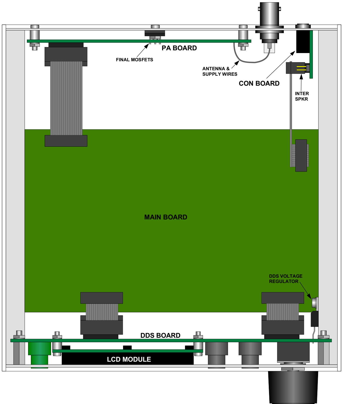
JUMA-TRX2 HF TRANSCEIVER Two band construction OH2NLT and OH7SV 2007
